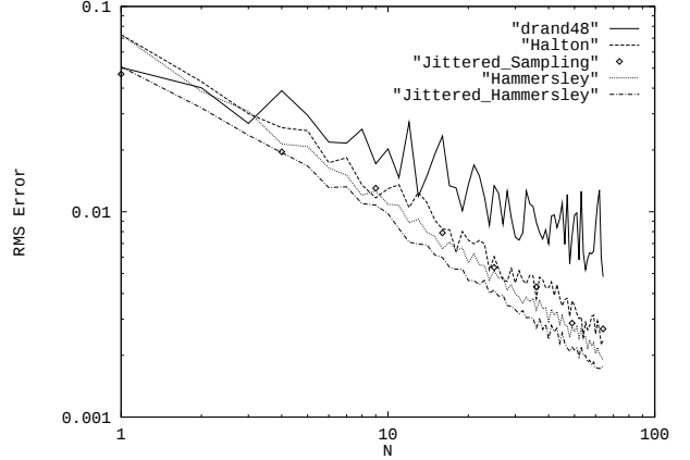
Figure 6: Convergence of different sampling patterns.
